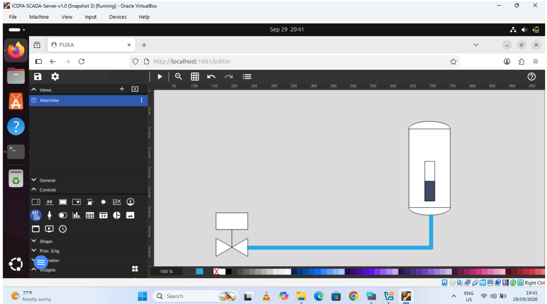
Caption: Figure 2 — FUXA HMI Canvas in Editor mode (2026WT_LAB05), showing neutral gray canvas, aligned process piping, tank asset, bar gauge (0–10 ft), and valve assembly.
